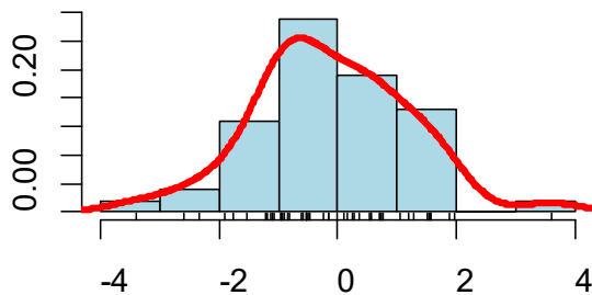
Fat tailed distributio
