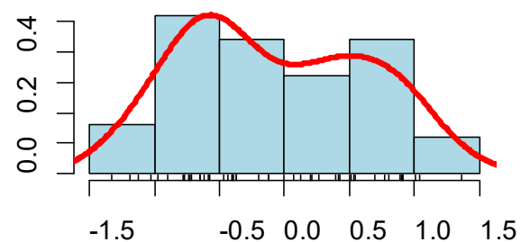
Fat tailed distributio
