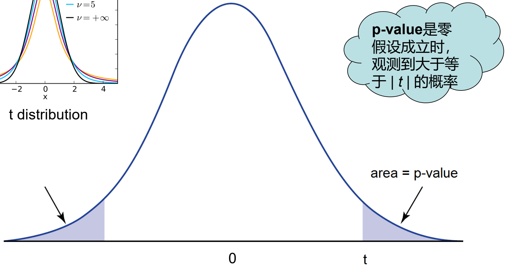
The distribution of the t-statistic under the null hypothesis
